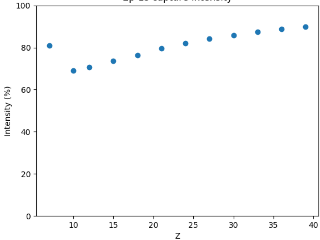
2p-1s capture intensity
