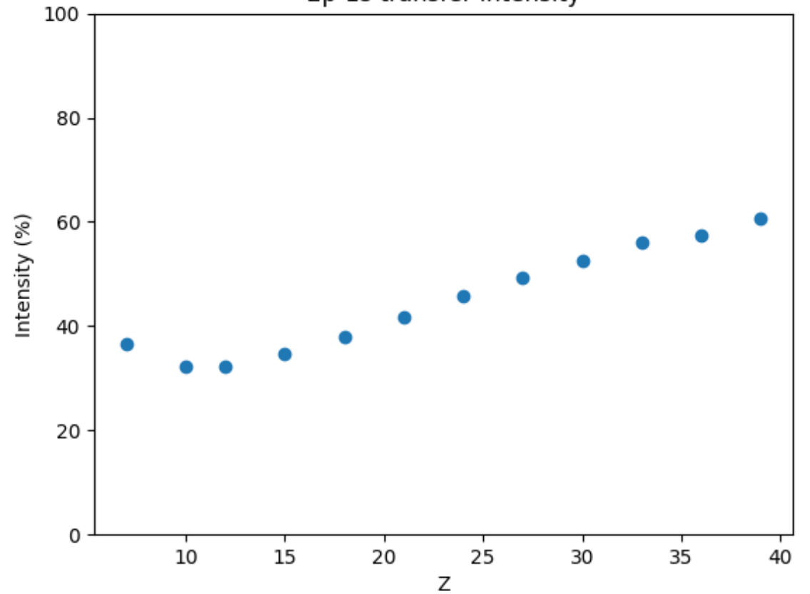
2p-1s transfer intensity
