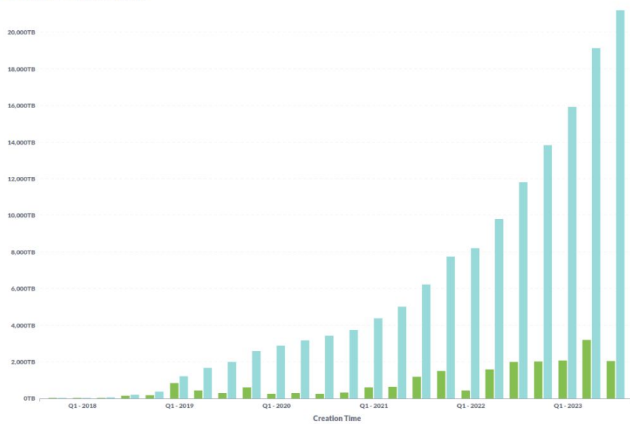
PSI Dataset Archive Statistics over Time
