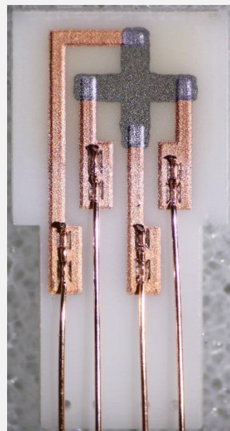
Ultrasonically bonded Cu wires
