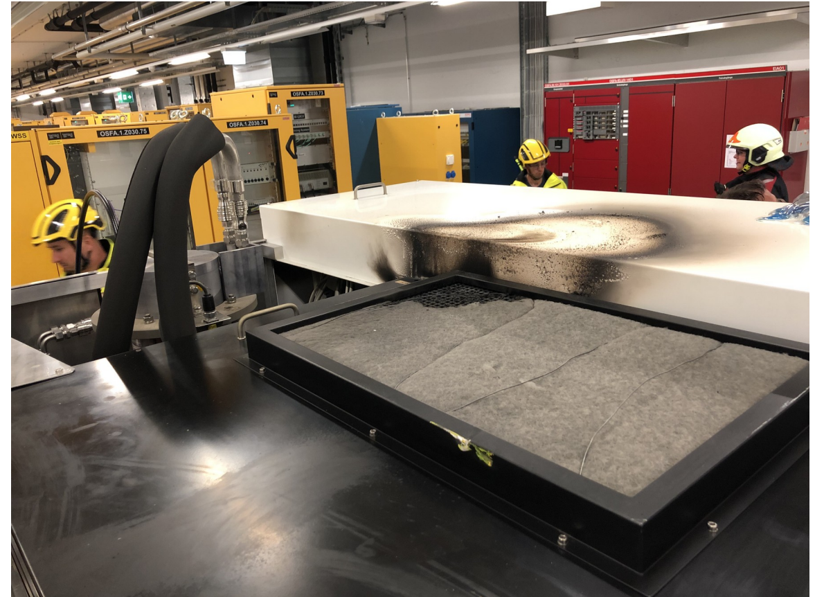
top cover
