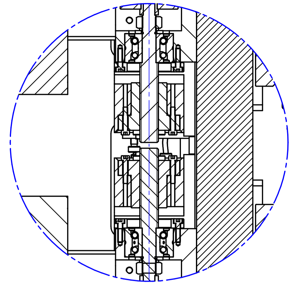
DETAIL C
