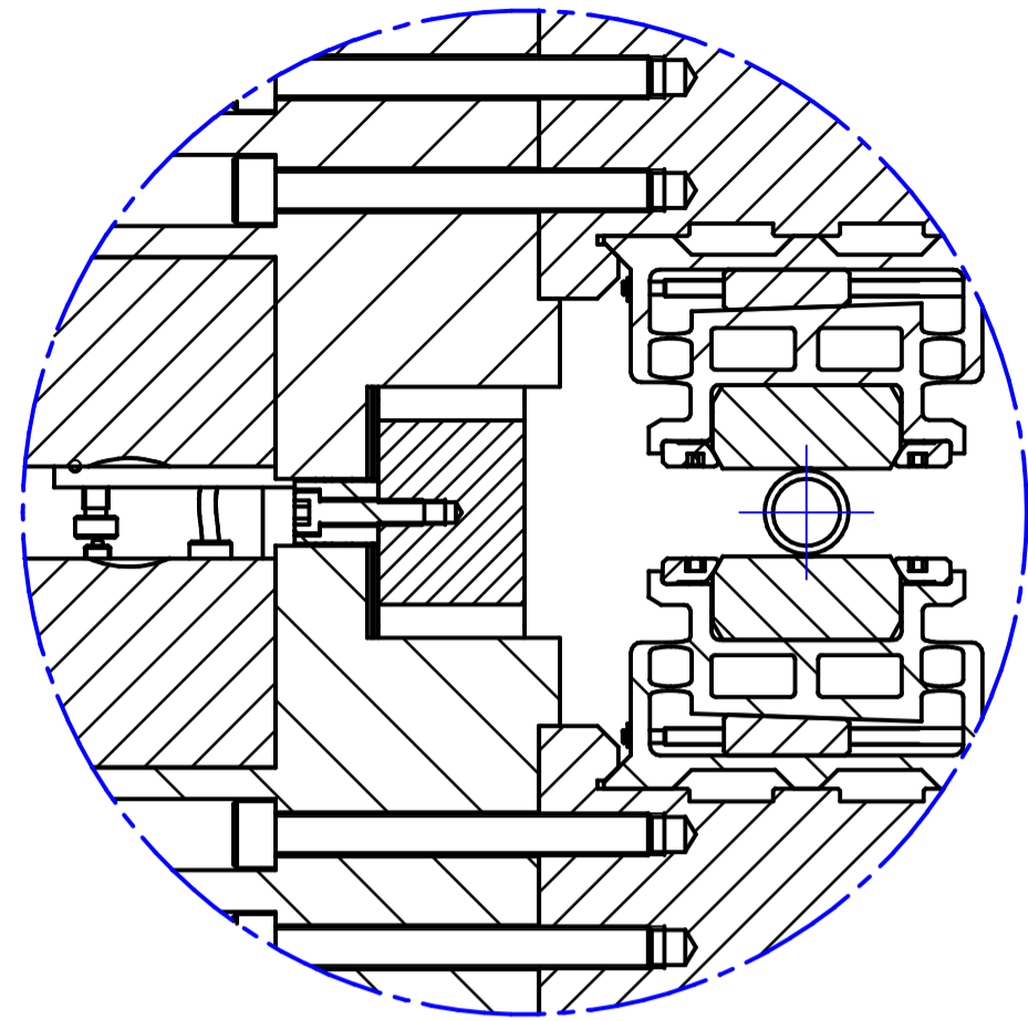
DETAIL D
