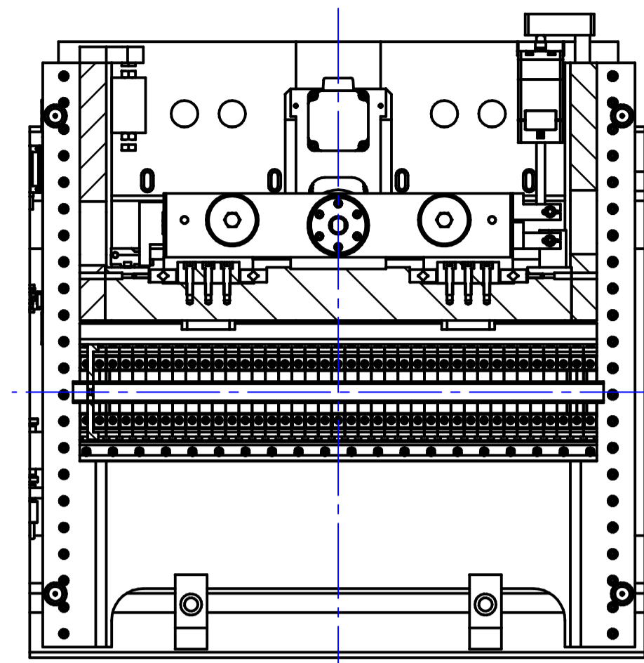
SECTION E-E
